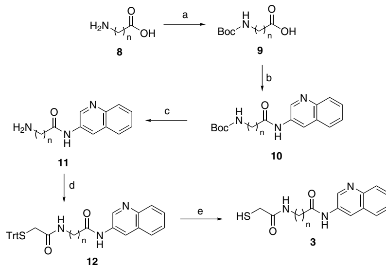
Scheme 2. Reagents and conditions: (a) (Boc) 2 O, NaOH, t -BuOH, 12 h (82–93%); (b) 3-aminoquinoline, HOBT, EDCI, DIEA, DCM, rt, 12 h (84–88%); (c) HCl/Et 2 O, 0 °C, 4 h; (d) S -tritylmercaptoacetic acid, HOBT, EDCI, DIEA, DCM, rt, 12 h (80–85%); (e) TFA, DIEA, DCM, 1 h (41–51%).
