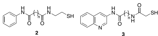
Figure 2. Mercaptoamide based non-hydroxamate HDAC inhibitors.
