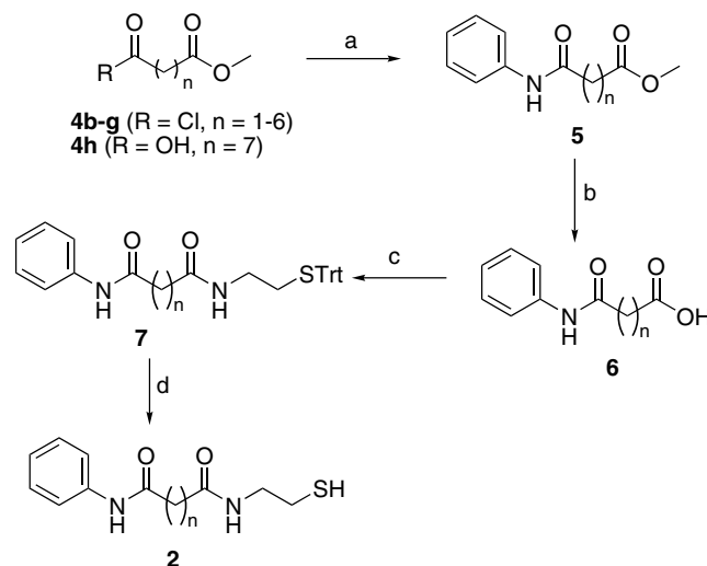
Scheme 1. Reagents and conditions: (a) aniline, DIEA, DCM, 0–10 °C for 10 min, rt for 30 min (83–85%) or EDCI, HOBT, DIEA, rt, 9 h (84–87%); (b) LiOH, EtOH, H 2 O, rt, 3 h (90–95%); (c) S -trityl cysteamine, EDCI, HOBT, DIEA, DCM, rt, 12 h (45–50%); (d) TFA, triisopropylsilane, DCM, 1 h (20–25%).
