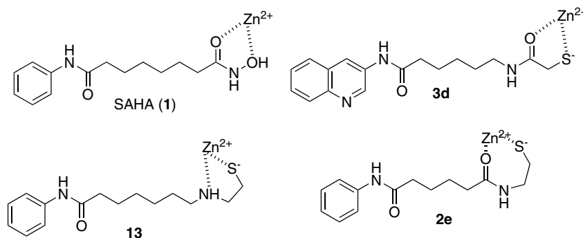
Figure 3. Bidentate chelation of hydroxamic acid in SAHA, mercaptoethylamine 13 and mercaptoamides 2e , 3d with Zn 2+ ion.
