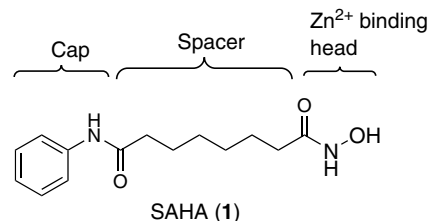
Figure 1. Structural motifs of HDAC inhibitor SAHA.
